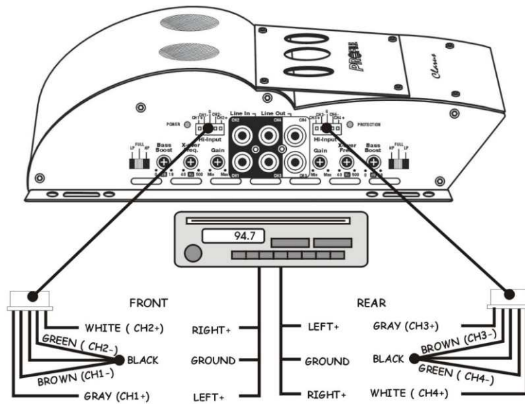
FOUR CHANNEL CONNECTIONS: COMMON GROUND RADIO
